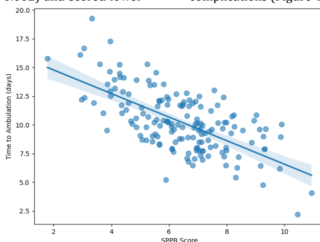
Figure 4. Linear Regression: SPPB Score vs. Time to Ambulation
