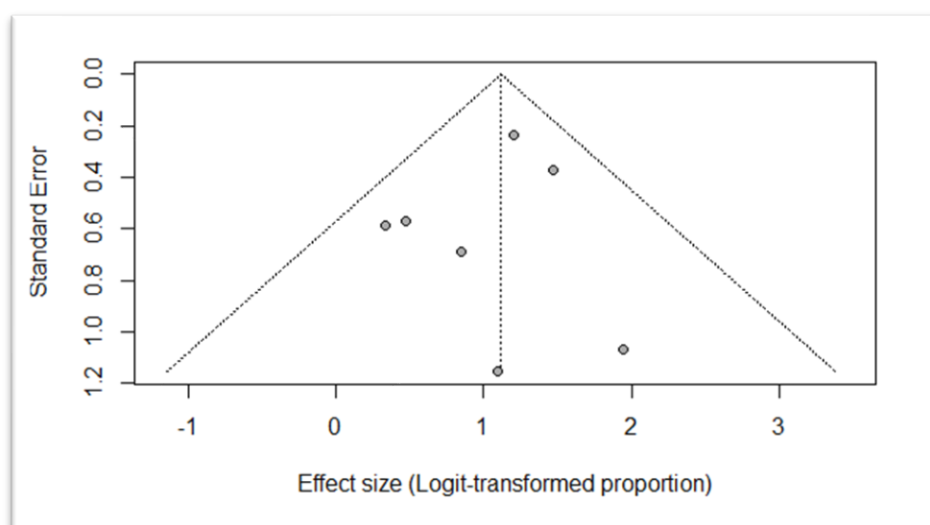
Figure(2) Funnel plot for Cureness Publication Bias
