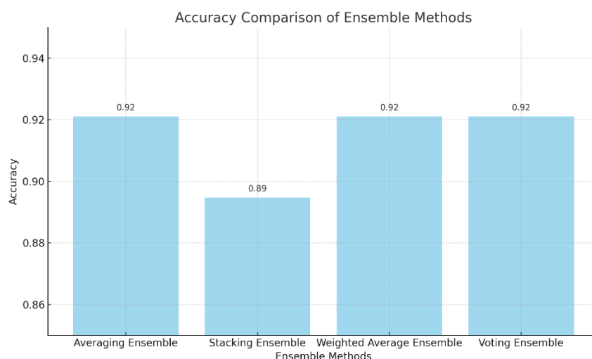
Figure 8: The Ensembling performance of the trained model
