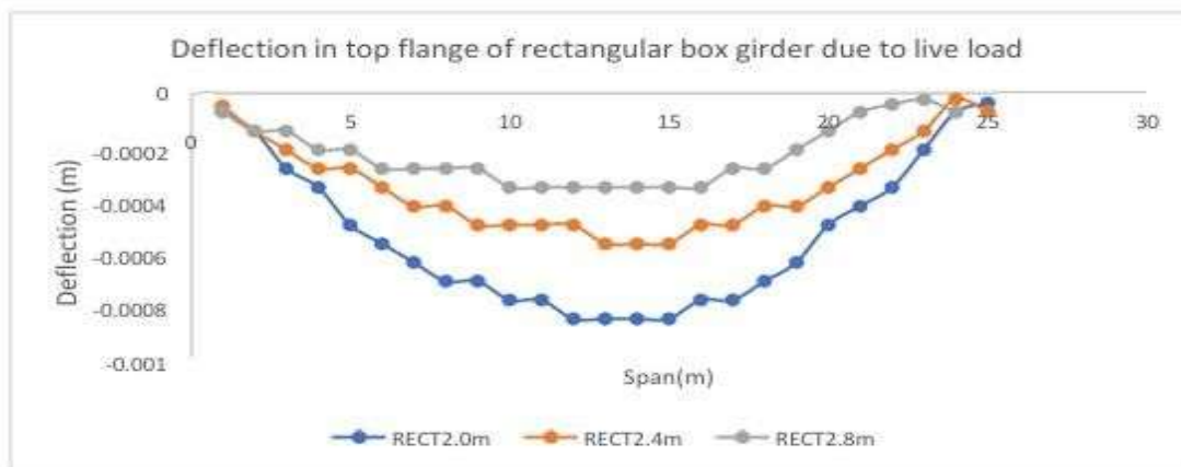
Figure 7.7 Deflection in top flange of rectangular box girder due to IRC 70 R live load
