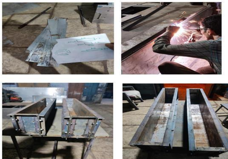
Figure No. 5.4 : Fabrication Of Reinforcement Formwork
