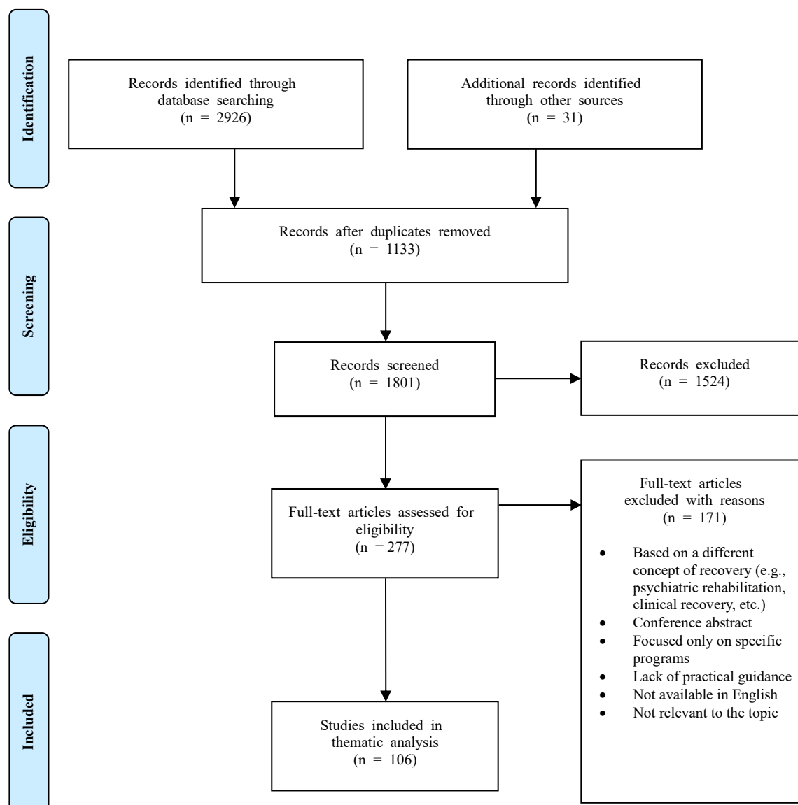
Figure 1. PRISMA-ScR flowchart
