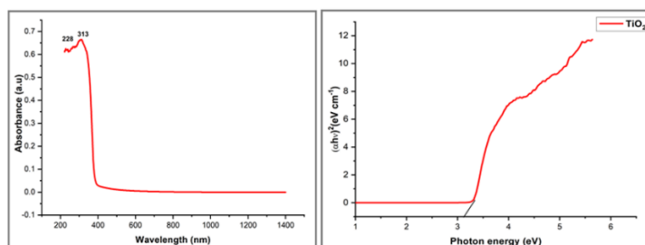
Fig. 1 (a) UV - Vis and (b) Tauc Plot pattern of C. p @ TiO 2 NPs
