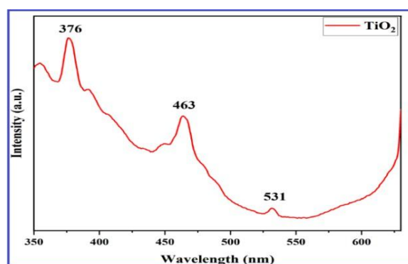
Fig. 2 Photoluminescence spectrum of C. p @ TiO 2 NPs
