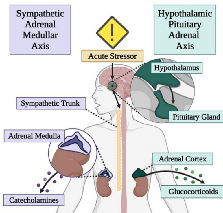
Figure 1: Stress pathways
